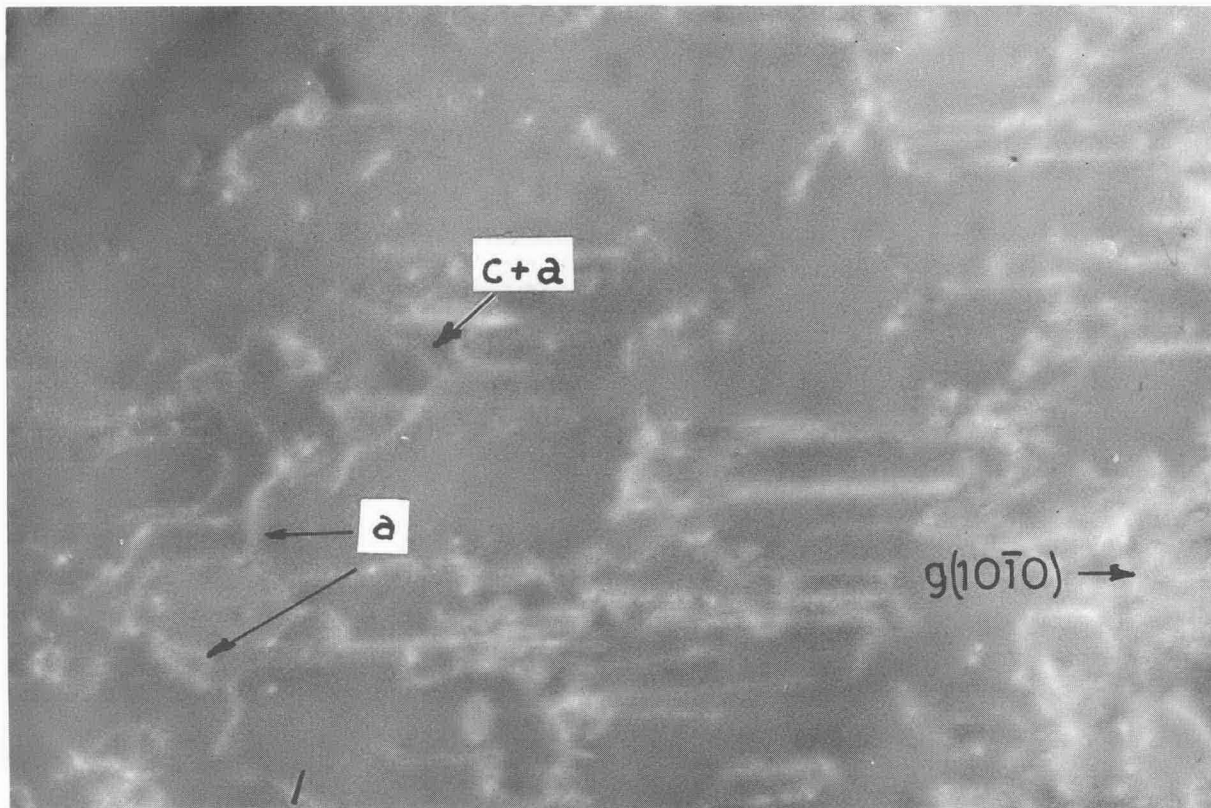
Fig. 13 - Electron Transmission Micrographs of Crystal ISR-12 Foil Showing Diffraction Contrast in Foil Cut Parallel to (11\bar{2}0) for (a) g(0002) and (b) g(10\bar{1}0) - Pyramidal Slip Lines are Delineated by Dislocations Having non-basal Burgers vectors. Mag. 37,500X
